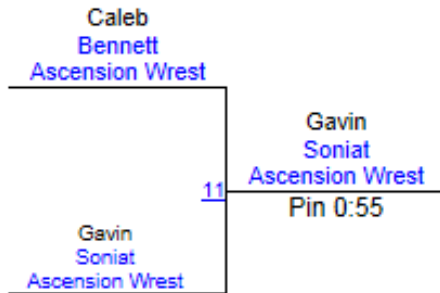
Round 1
