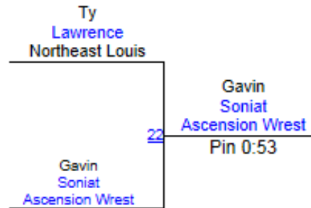
Round 2
