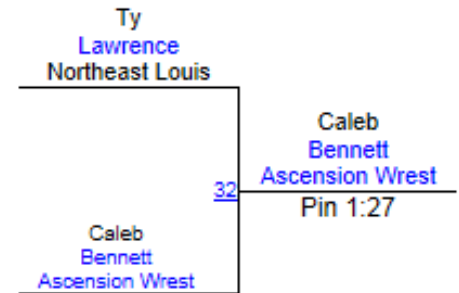
Round 3
