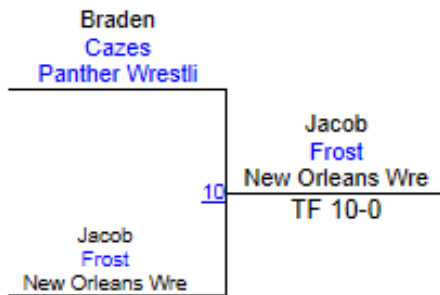
Round 1
