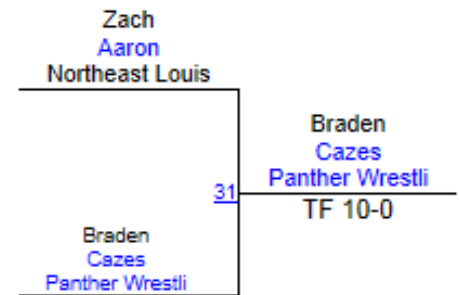
Round 3
