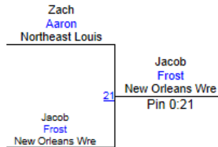
Round 2
